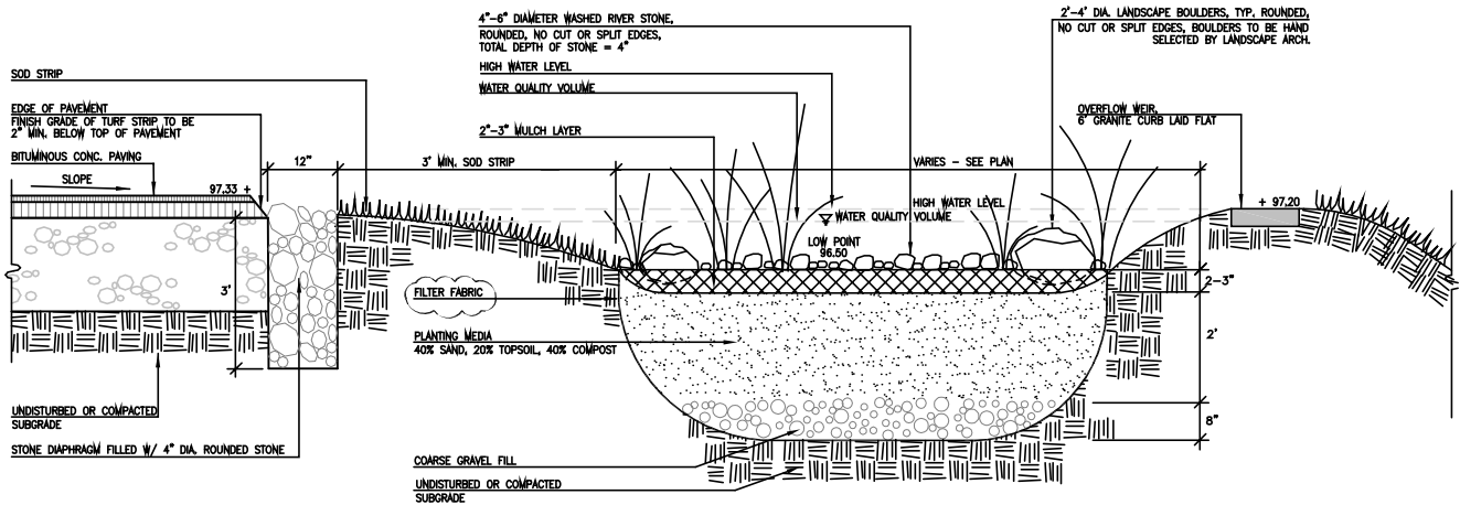
2 Rain Garden L5 Not To Scale
