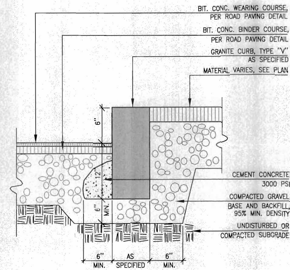
3 Granite Curb
