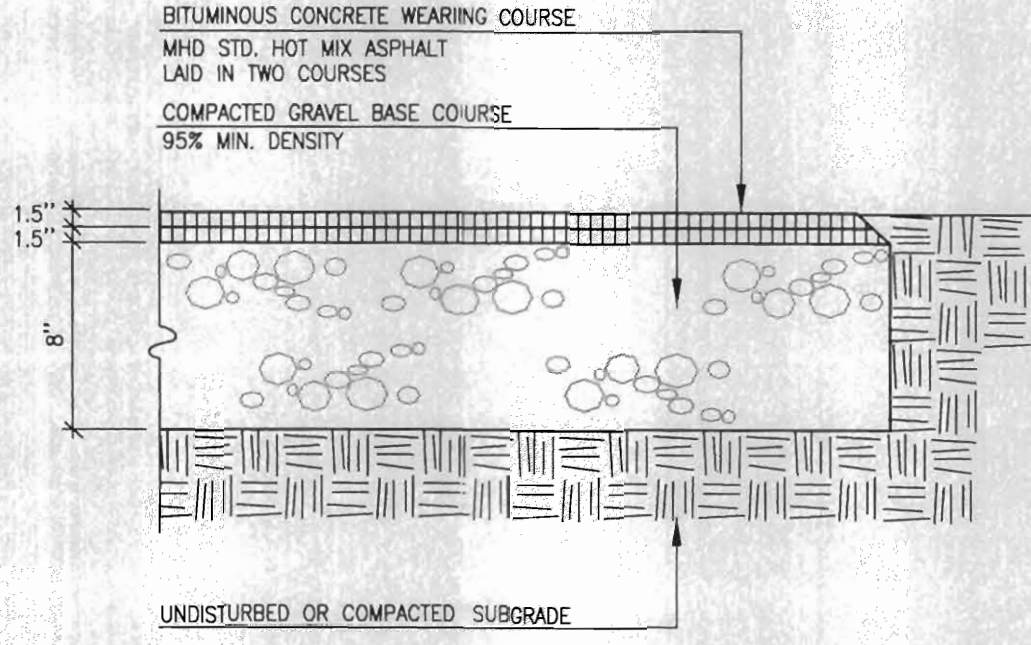
2 Bit. Conc. Walk Paving
