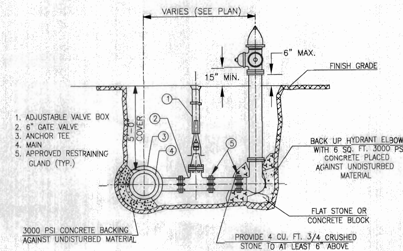
8 Hydrant Installation
