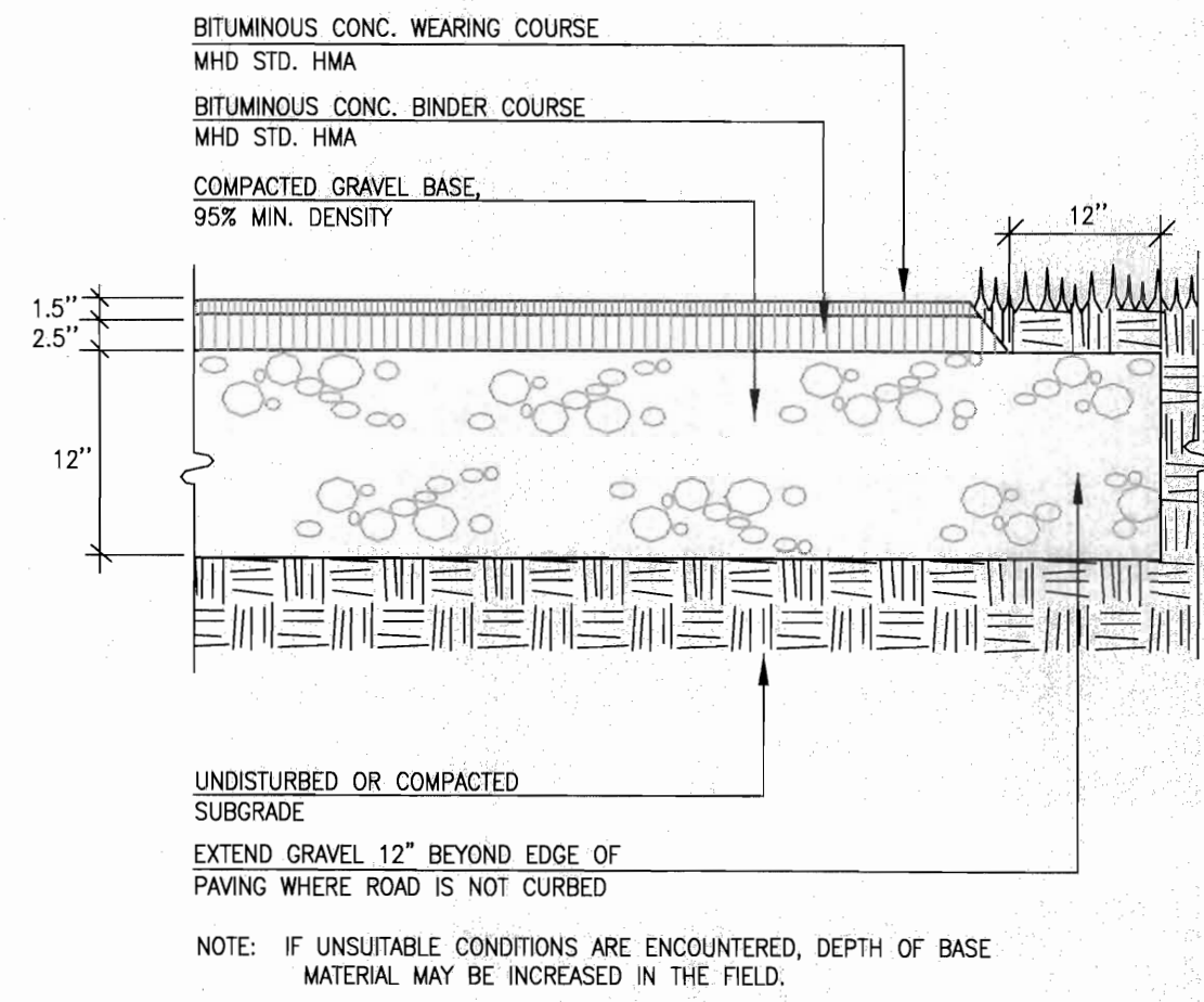
1 Bit. Conc. Road Paving
