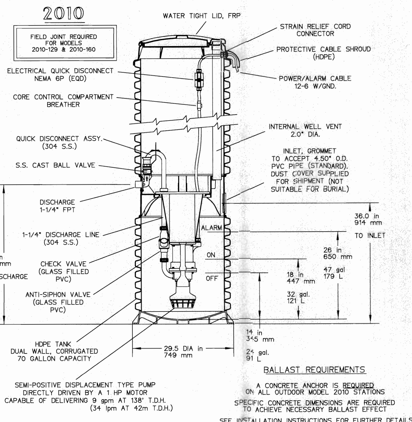
11 EONE Pump System Typical Detail
