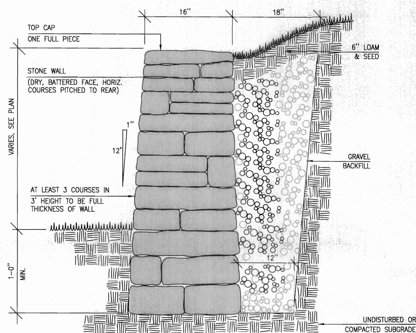
5 Stone Retaining Wall
