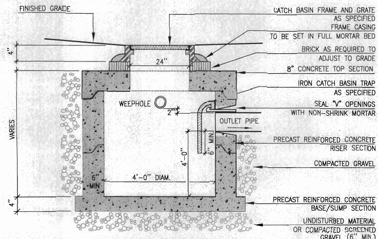
6 Catch Basin
