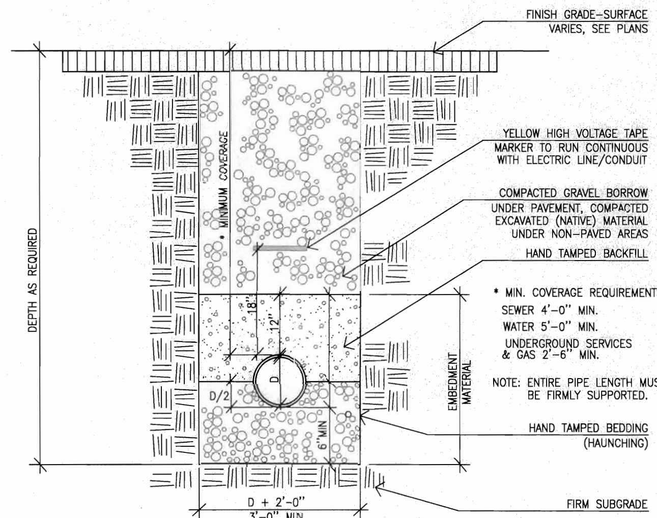
10 Typical Utility Trench
