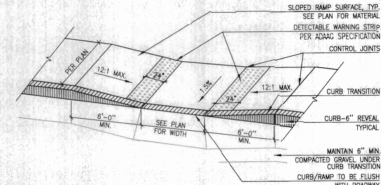
4 Sidewalk Ramp Transition
