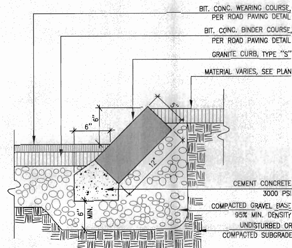
7 Slope Granite Curb
